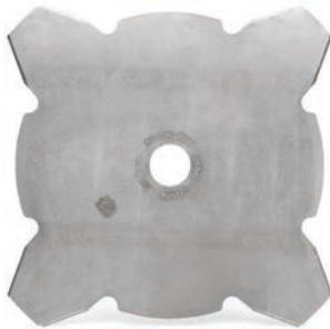
GRASS BLADE - 4 TOOTH, Ø 255MM, 1" ARBOR 578 44 37-01
